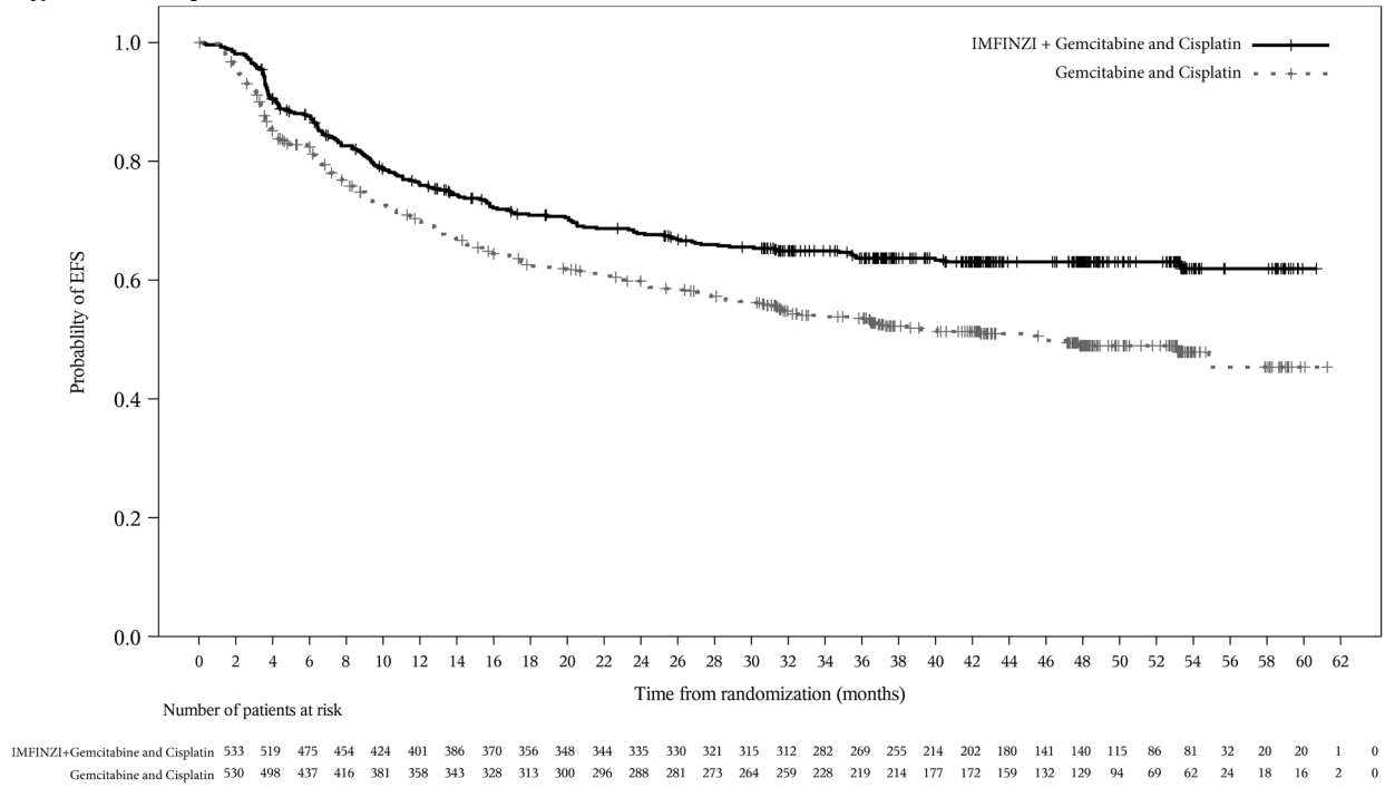
Figure 8. Kaplan-Meier Curve of EFS
