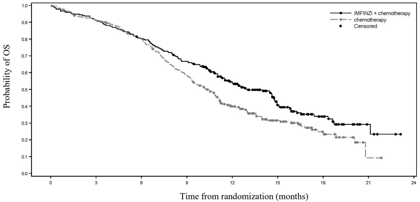
Figure 5. Kaplan-Meier Curves of OS in the CASPIAN Study
