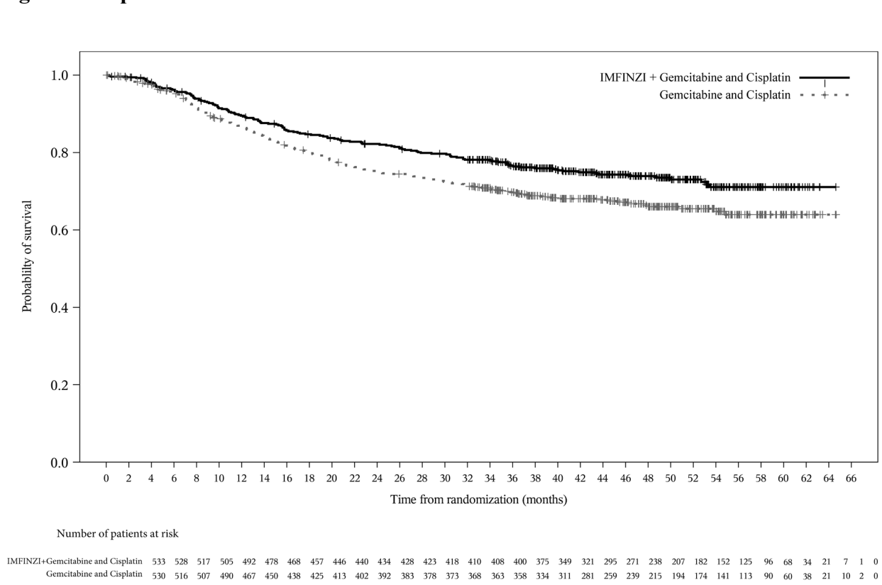
Figure 9. Kaplan-Meier Curve of OS
