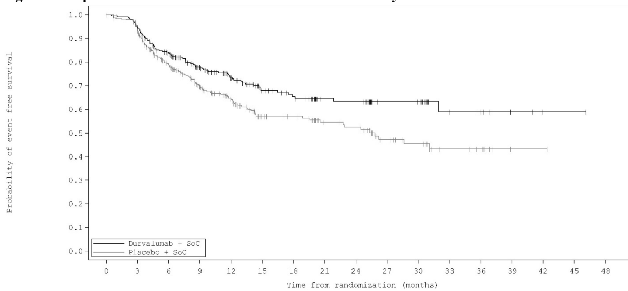
Figure 1. Kaplan-Meier Curves of EFS in the AEGEAN Study
