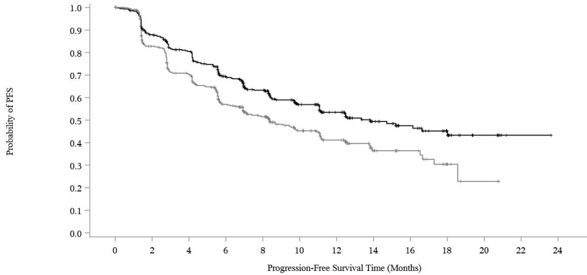
Figure 2: K-M Estimates for PFS based on BICR Assessment – ITT
